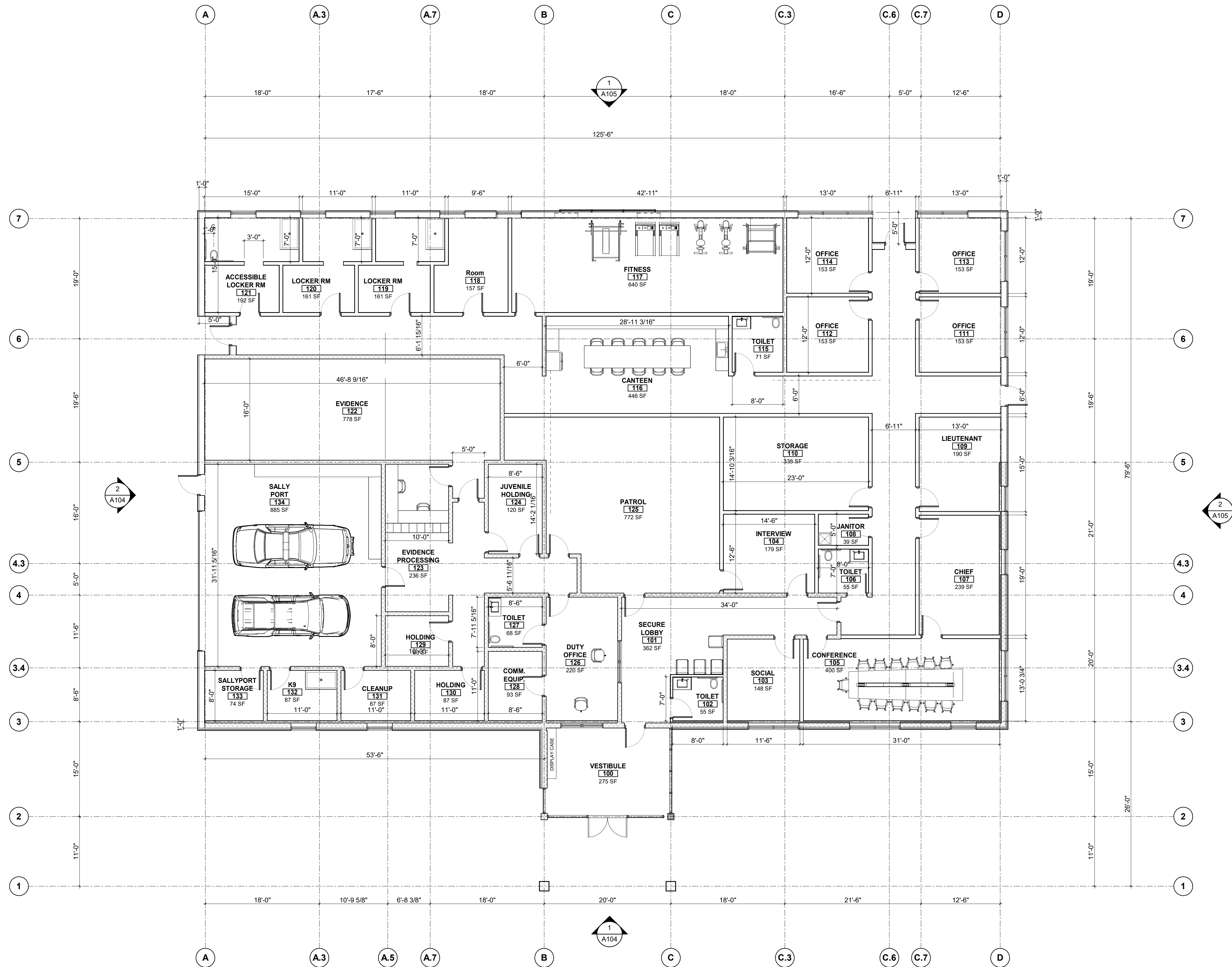
1 FIRST FLOOR DIMENSION PLAN 1/8" = 1'-0"
