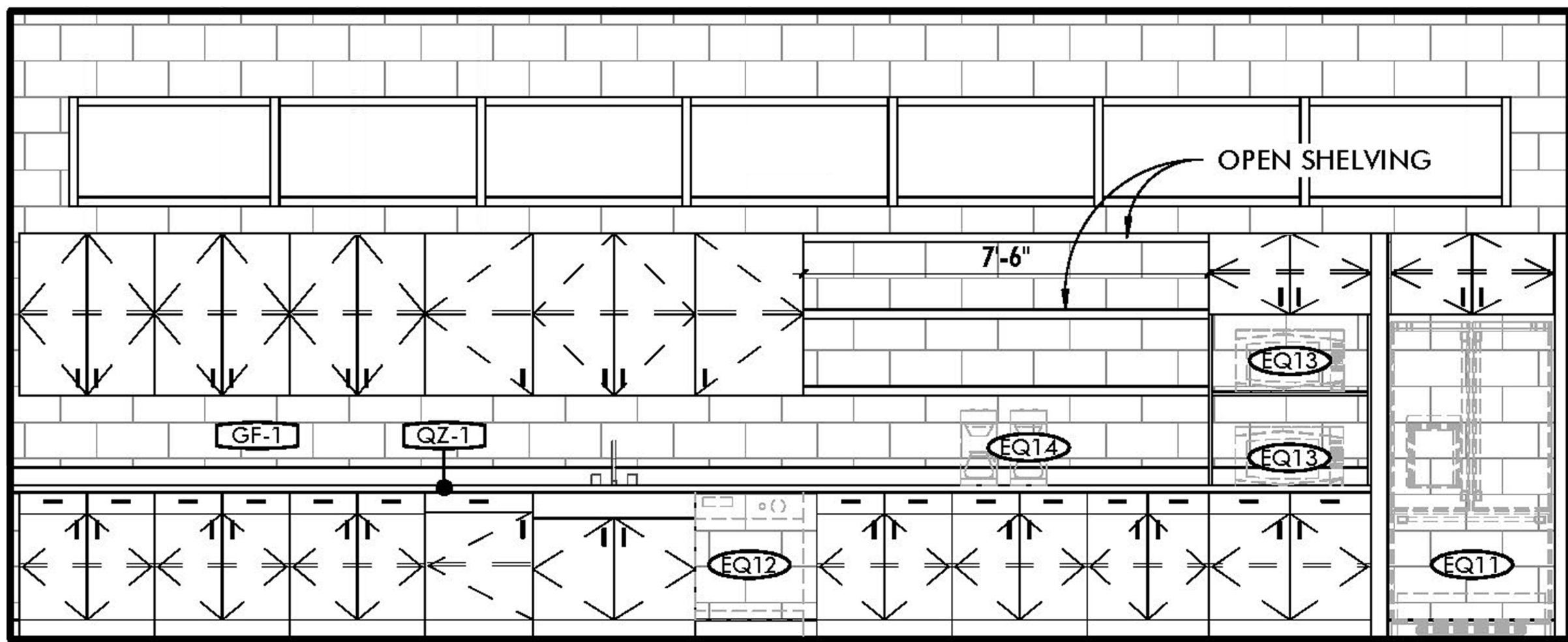
Canteen 123 - North Elevation
